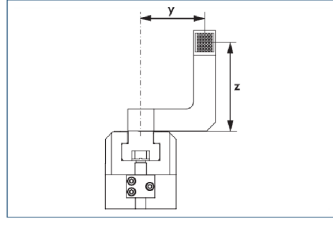
Maximum permitted finger offset
